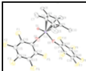
Fig. 1. The asymmetric unit of the title compound ( I ), showing the atom-labelling scheme. Displacement ellipsoids are drawn at the 20% probability level. H atoms are omitted for clarity.
