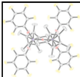
Fig. 2. The molecular structure of the title compound ( I ). Displacement ellipsoids are drawn at the 20% probability level. H atoms are omitted for clarity.
